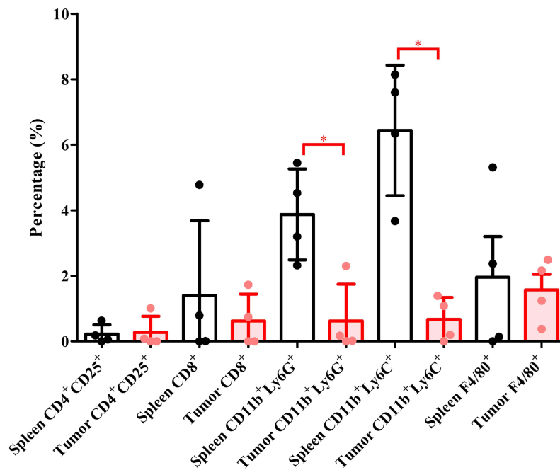
Figure 5 MDSCs in spleen and tumor samples from PDX-implanted nude mice. Intrasplenic immune cells are represented as circulatory immune cells, and intratumor immune cells correspond to the tumor microenvironment. * P < 0.05 .
