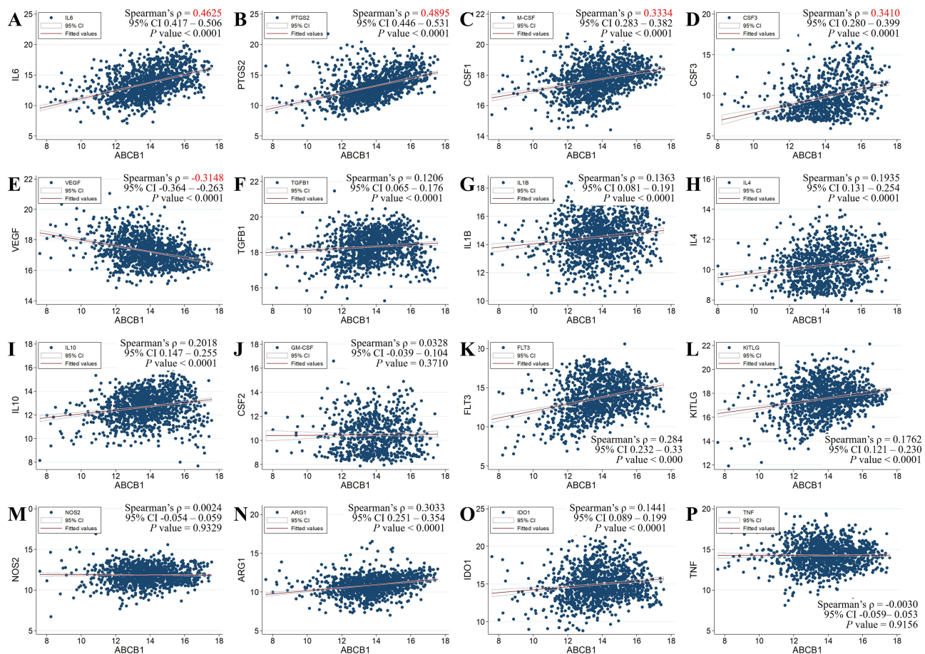
Figure 2 Correlation between the ABCB1 gene and immune genes in 1217 breast cancer samples from the TCGA. (A) IL6 , (B) PTGS2 , (C) CSF1 (M-CSF), (D) CSF3 , (E) VEGFA , (F) TGFB1 , (G) IL1B , (H) IL4 , (I) IL10 , (J) CSF2 (GM-CSF), (K) FLT3 , (L) KITLG , (M) NOS2 , (N) ARG1 , (O) IDO1 , and (P) TNF . MDSC, myeloid-derived suppressor cell; TCGA, The Cancer Genome Atlas.
